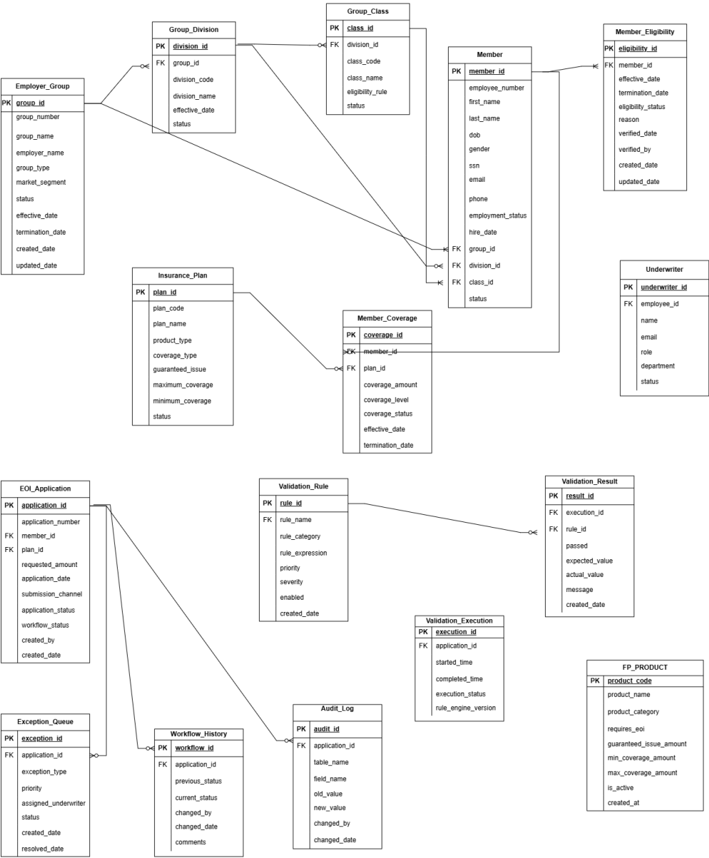
Draft Entity Model For EOI Process Validation
